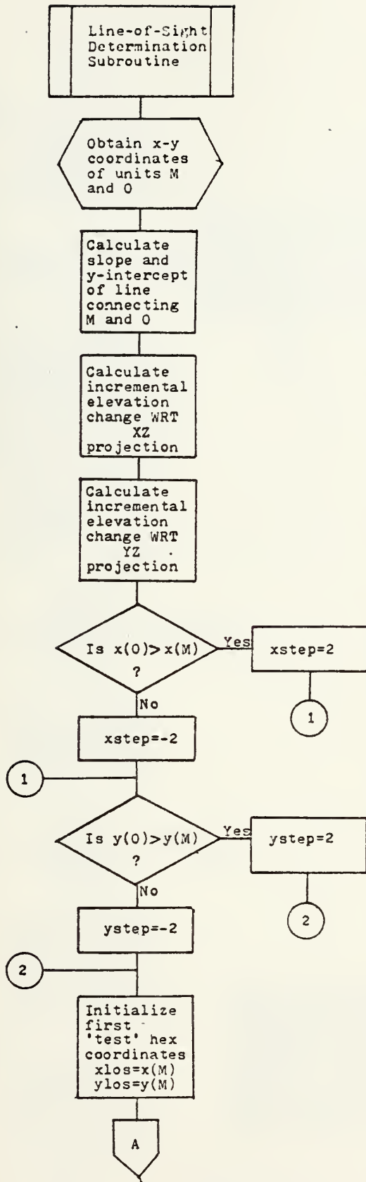
FIGURE V.9 FLOWCHART OF LINE-OF-SIGHT DETERMINATION SUBROUTINE
